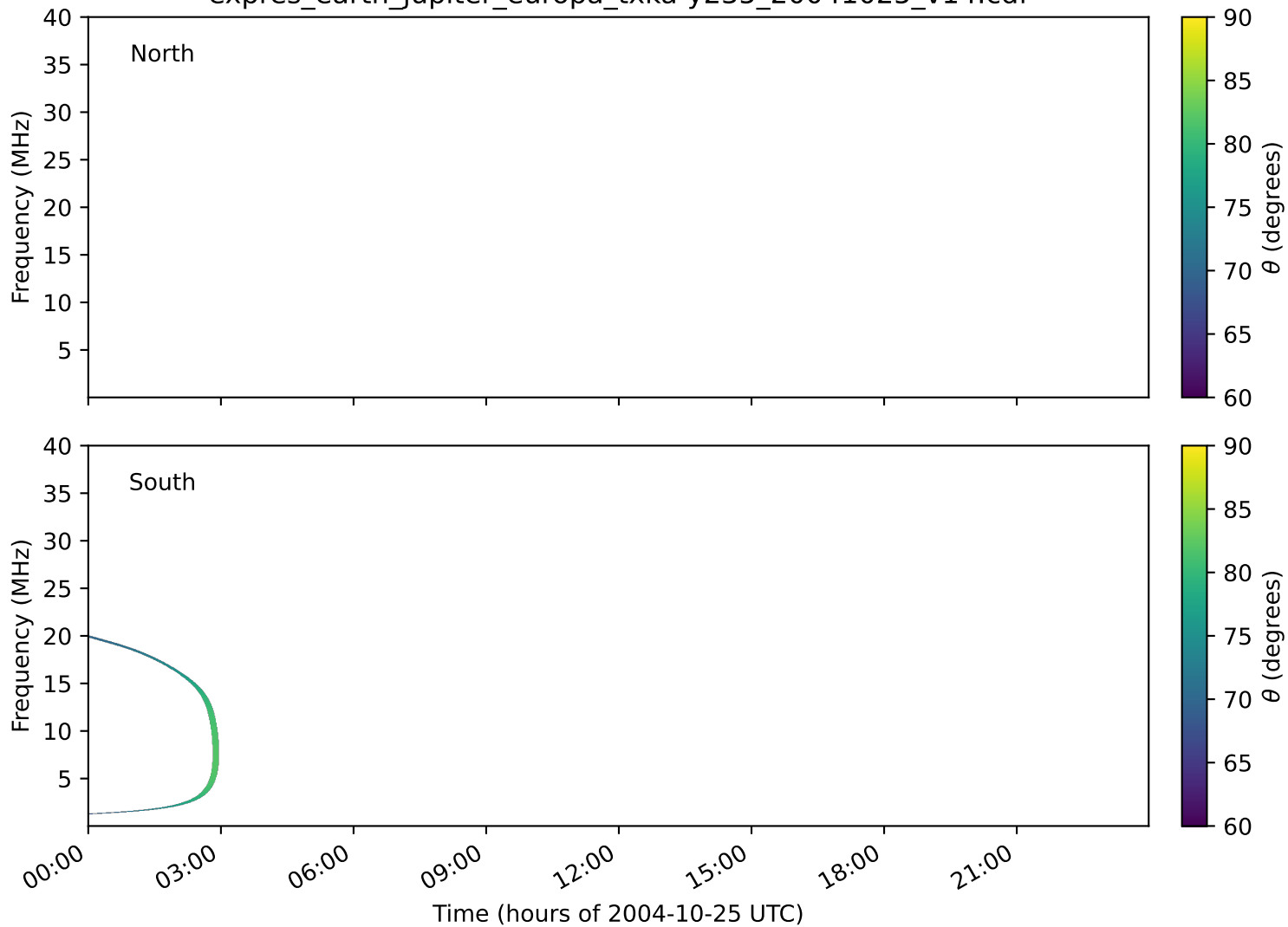
expres_earth_jupiter_europa_txka-y235_20041025_v14.cdf
