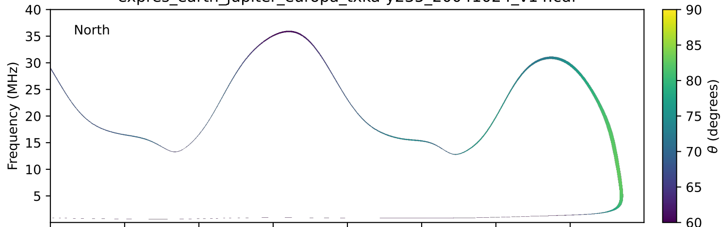
expres_earth_jupiter_europa_txka-y235_20041024_v14.cdf
