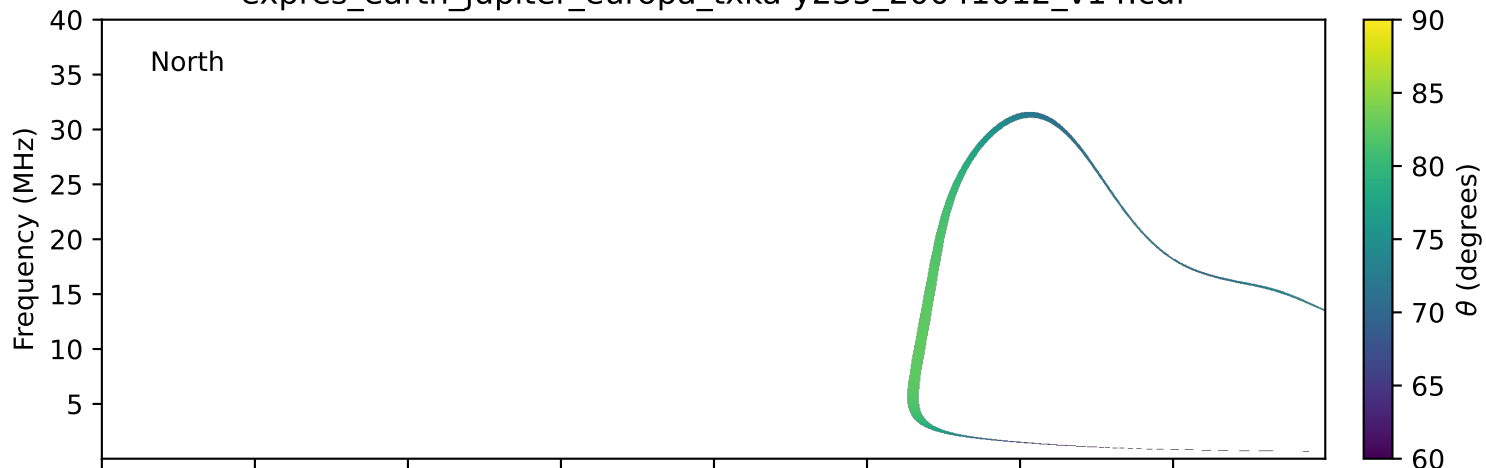
expres_earth_jupiter_europa_txka-y235_20041012_v14.cdf
