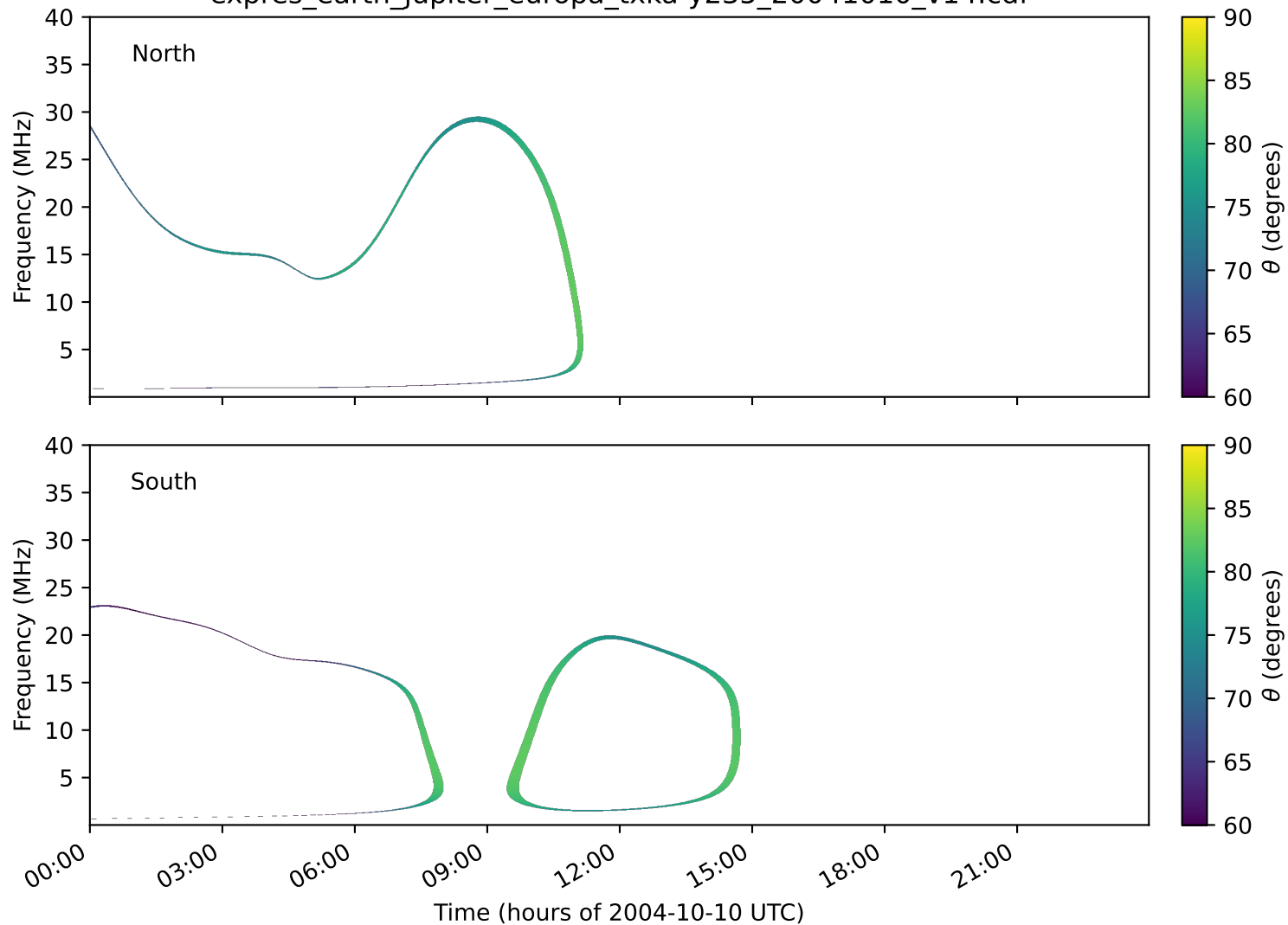
expres_earth_jupiter_europa_txka-y235_20041010_v14.cdf
