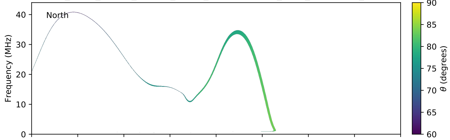
expres_earth_jupiter_europa_jrm09_lossc-wid1deg_3kev_20041028_v11.cdf
