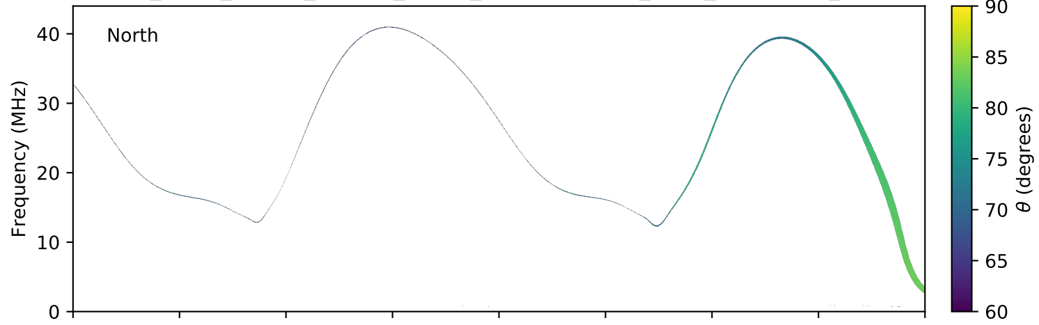
expres_earth_jupiter_europa_jrm09_lossc-wid1deg_3kev_20041024_v11.cdf
