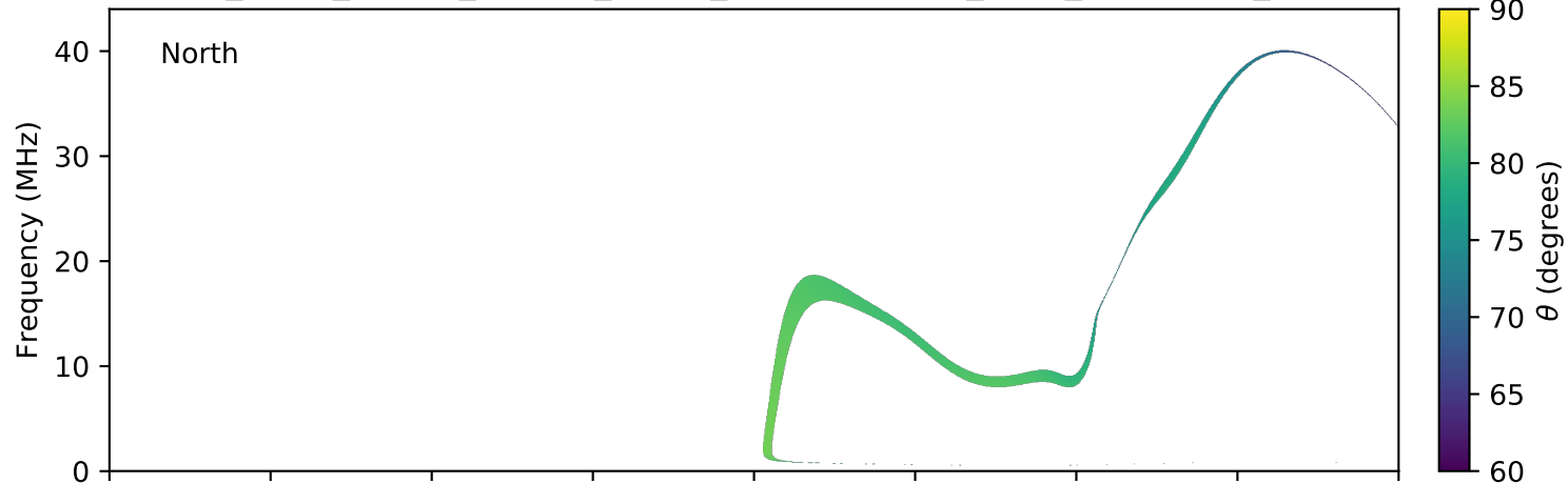
expres_earth_jupiter_europa_jrm09_lossc-wid1deg_3kev_20041023_v11.cdf
