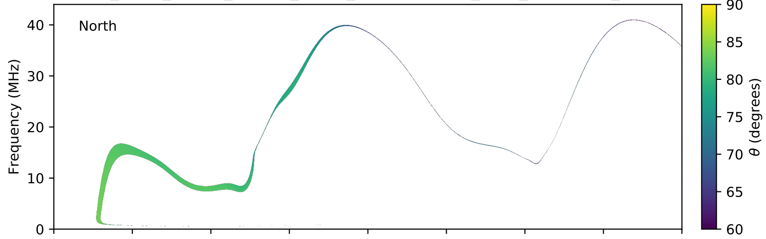
expres_earth_jupiter_europa_jrm09_lossc-wid1deg_3kev_20041016_v11.cdf
