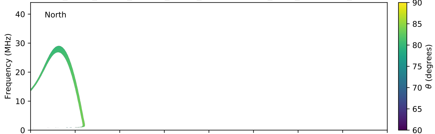
expres_earth_jupiter_europa_jrm09_lossc-wid1deg_3kev_20041014_v11.cdf
