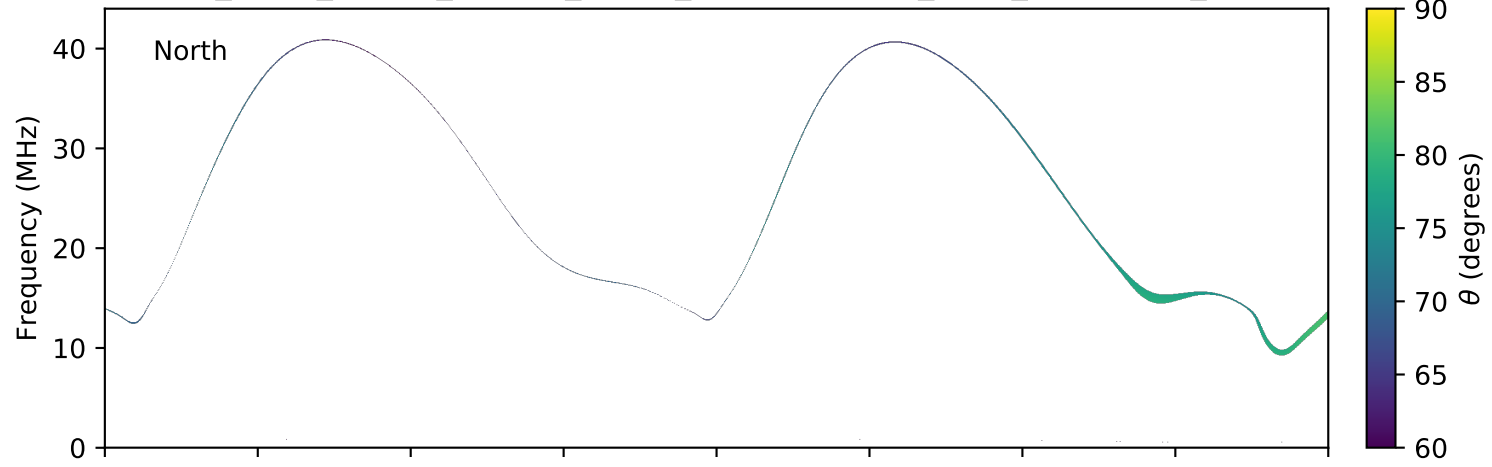
expres_earth_jupiter_europa_jrm09_lossc-wid1deg_3kev_20041013_v11.cdf
