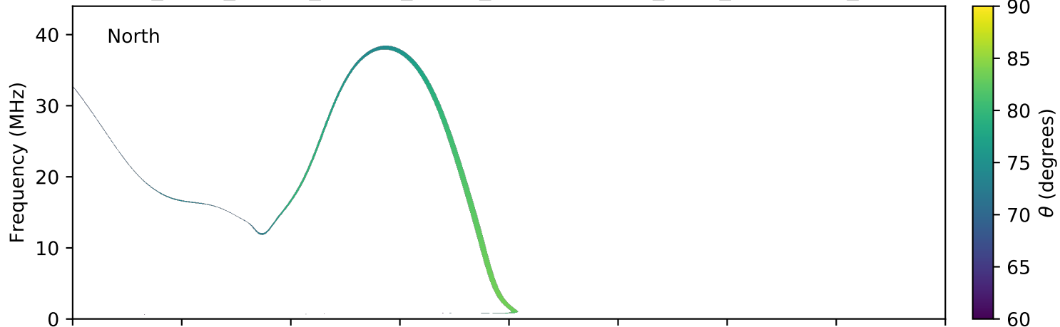
expres_earth_jupiter_europa_jrm09_lossc-wid1deg_3kev_20041010_v11.cdf
