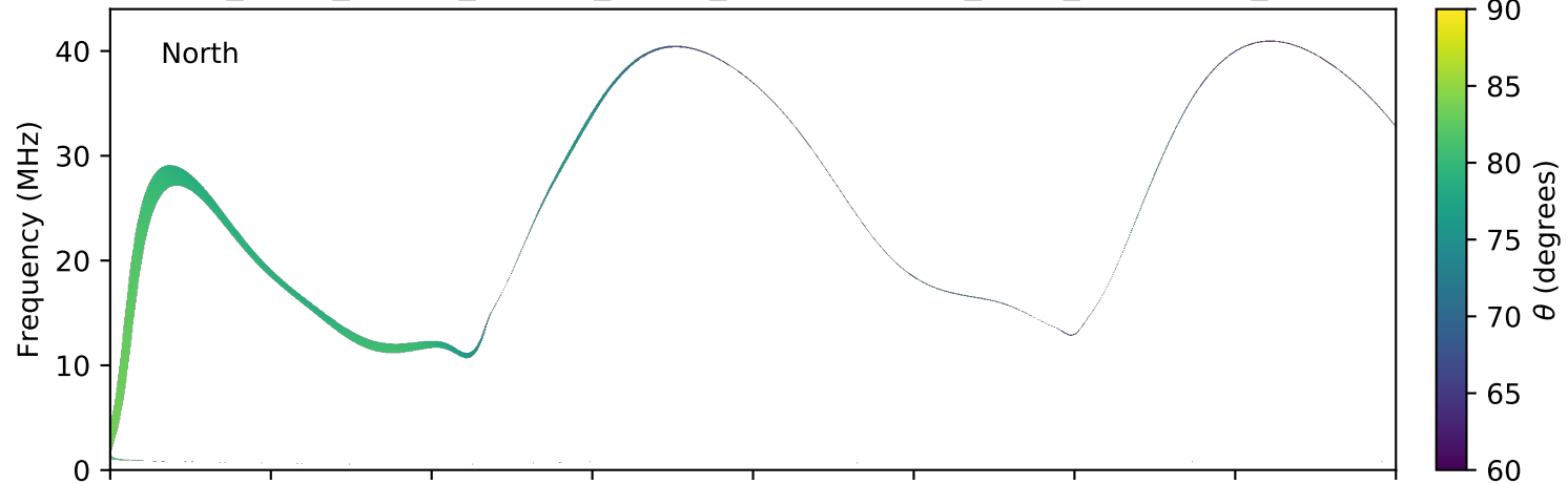
expres_earth_jupiter_europa_jrm09_lossc-wid1deg_3kev_20041009_v11.cdf
