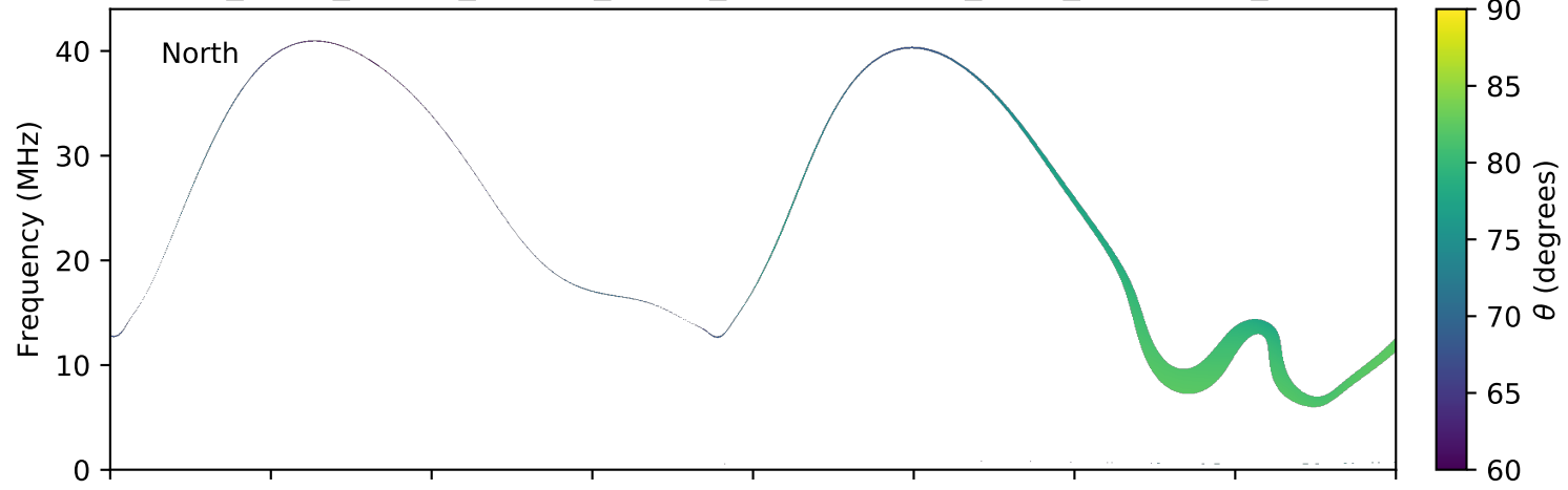
expres_earth_jupiter_europa_jrm09_lossc-wid1deg_3kev_20041006_v11.cdf
