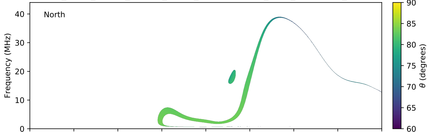
expres_earth_jupiter_europa_jrm09_lossc-wid1deg_3kev_20041005_v11.cdf
