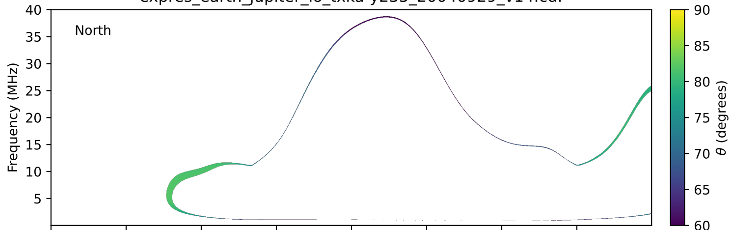
expres_earth_jupiter_io_txka-y235_20040929_v14.cdf
