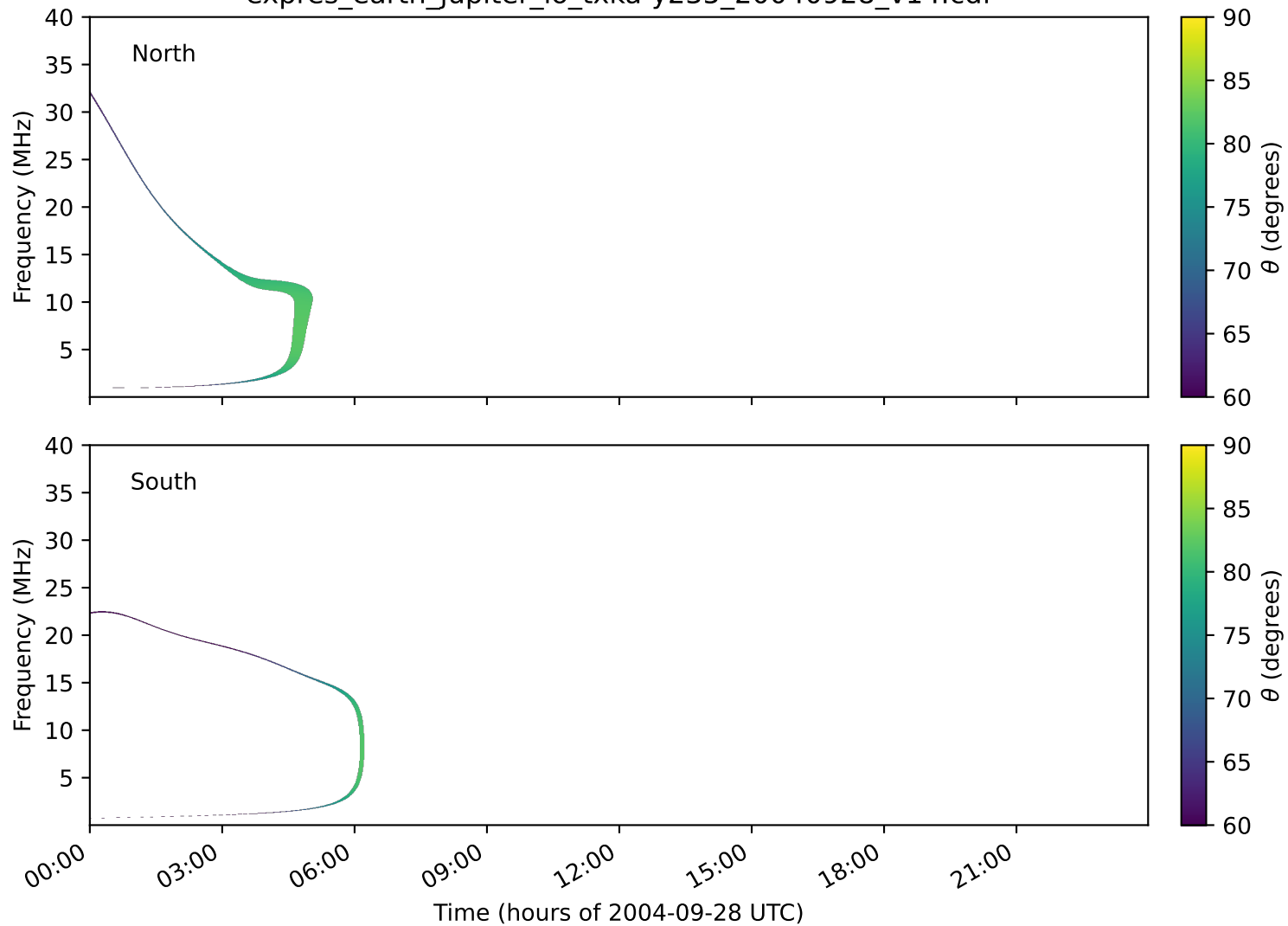
expres_earth_jupiter_io_txka-y235_20040928_v14.cdf
