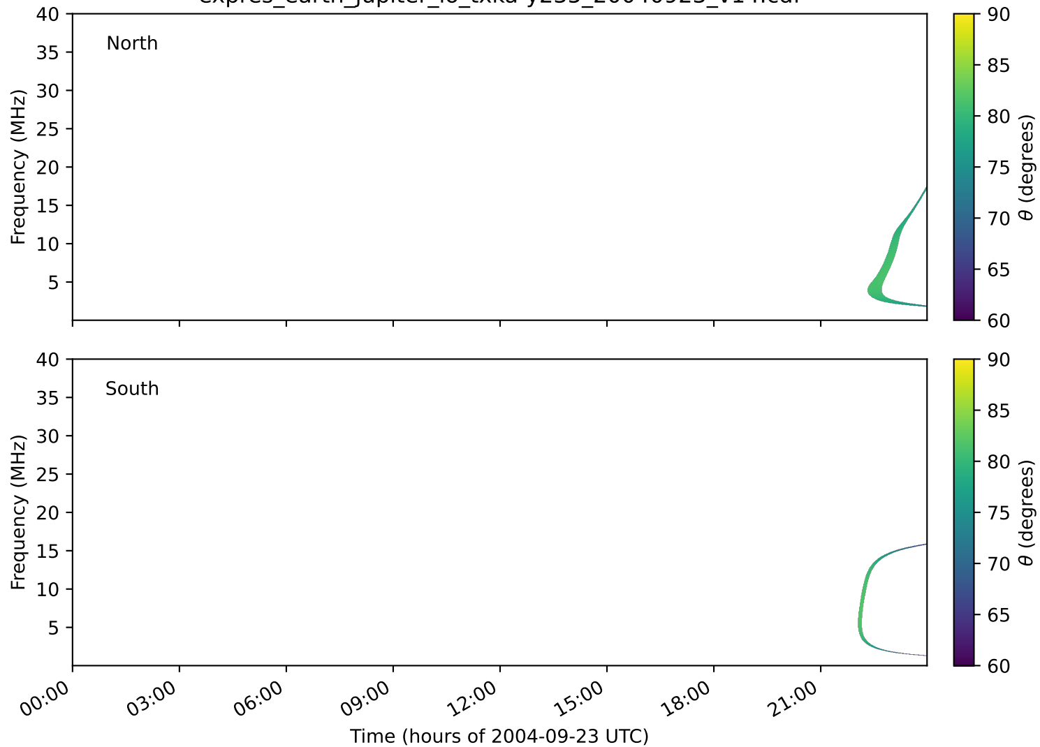
expres_earth_jupiter_io_txka-y235_20040923_v14.cdf
