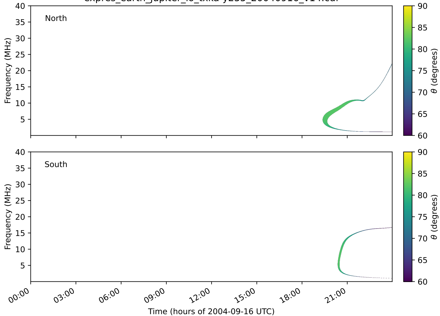
expres_earth_jupiter_io_txka-y235_20040916_v14.cdf
