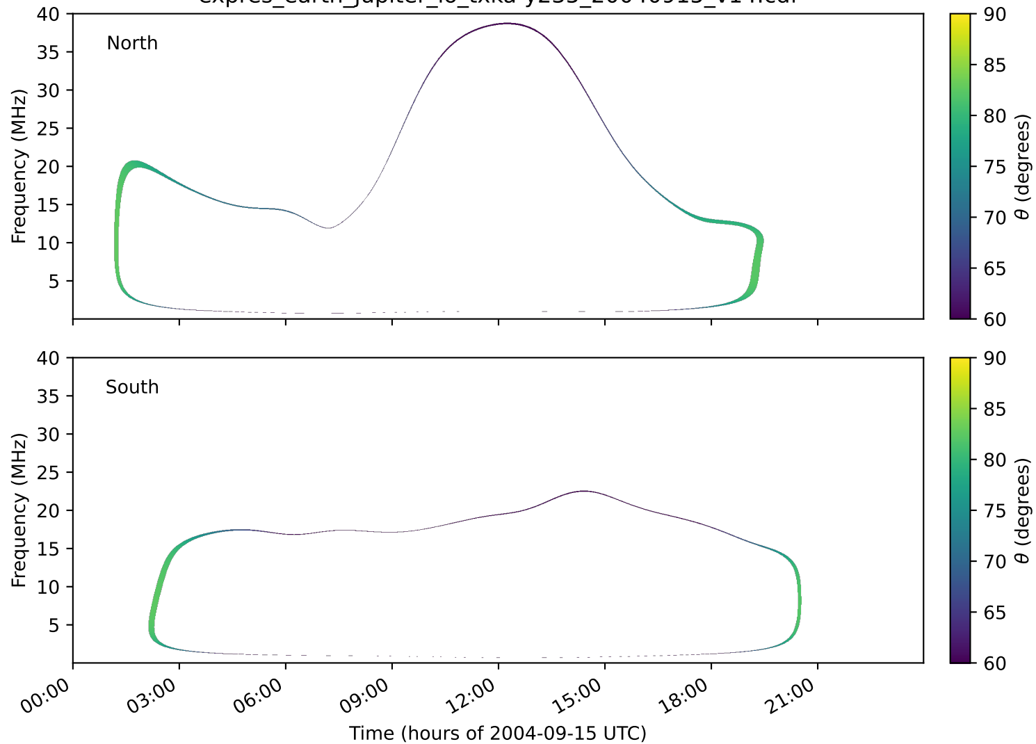
expres_earth_jupiter_io_txka-y235_20040915_v14.cdf
