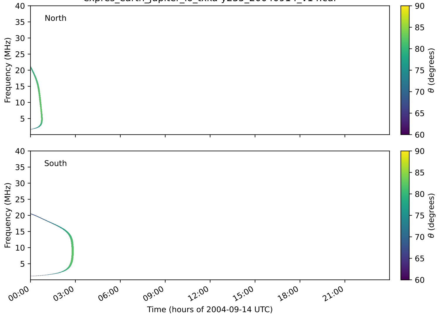
expres_earth_jupiter_io_txka-y235_20040914_v14.cdf
