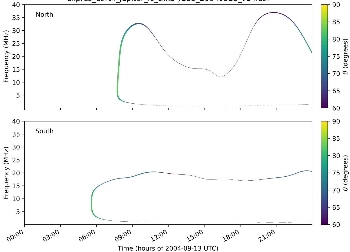
expres_earth_jupiter_io_txka-y235_20040913_v14.cdf
