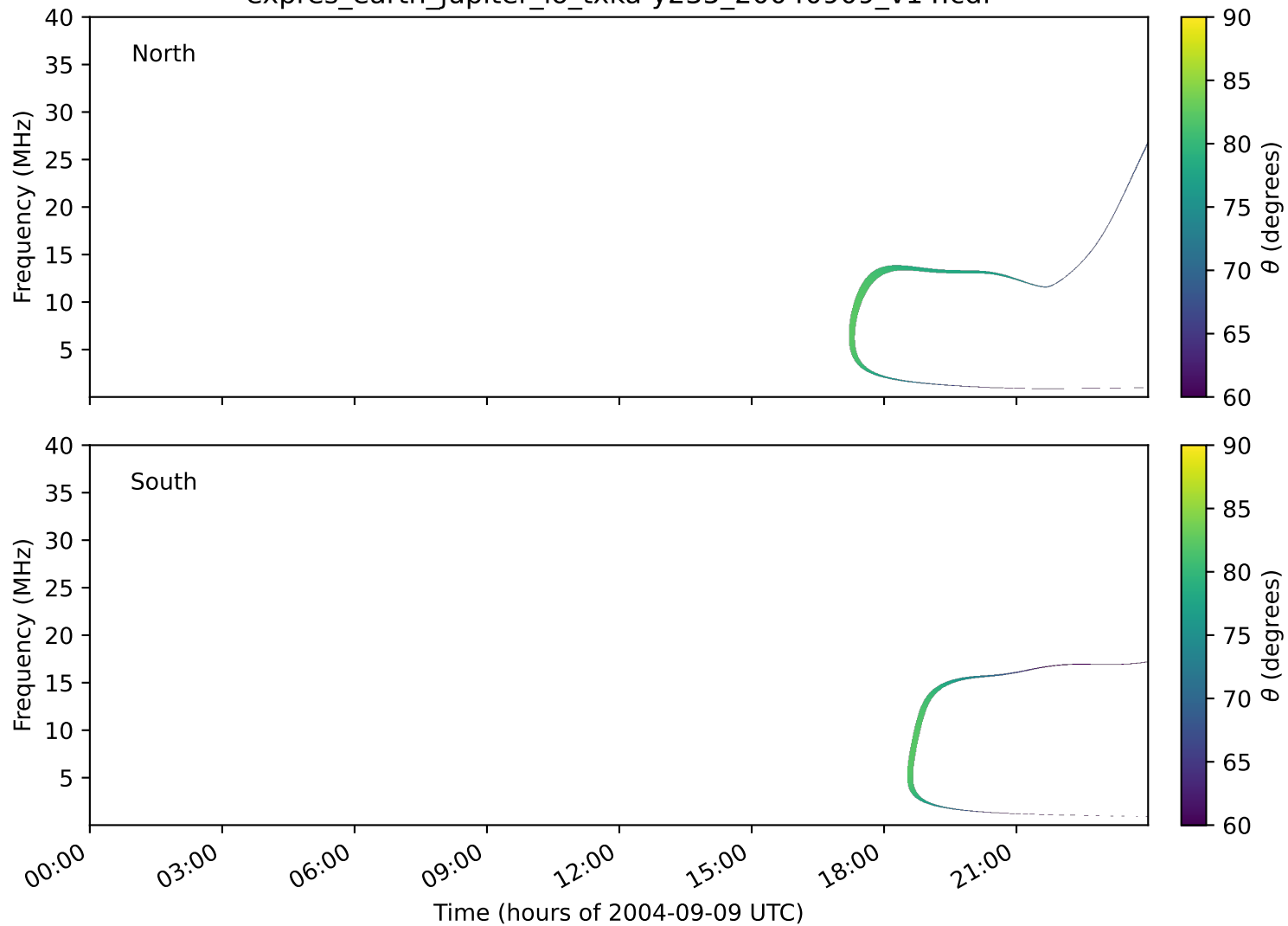
expres_earth_jupiter_io_txka-y235_20040909_v14.cdf
