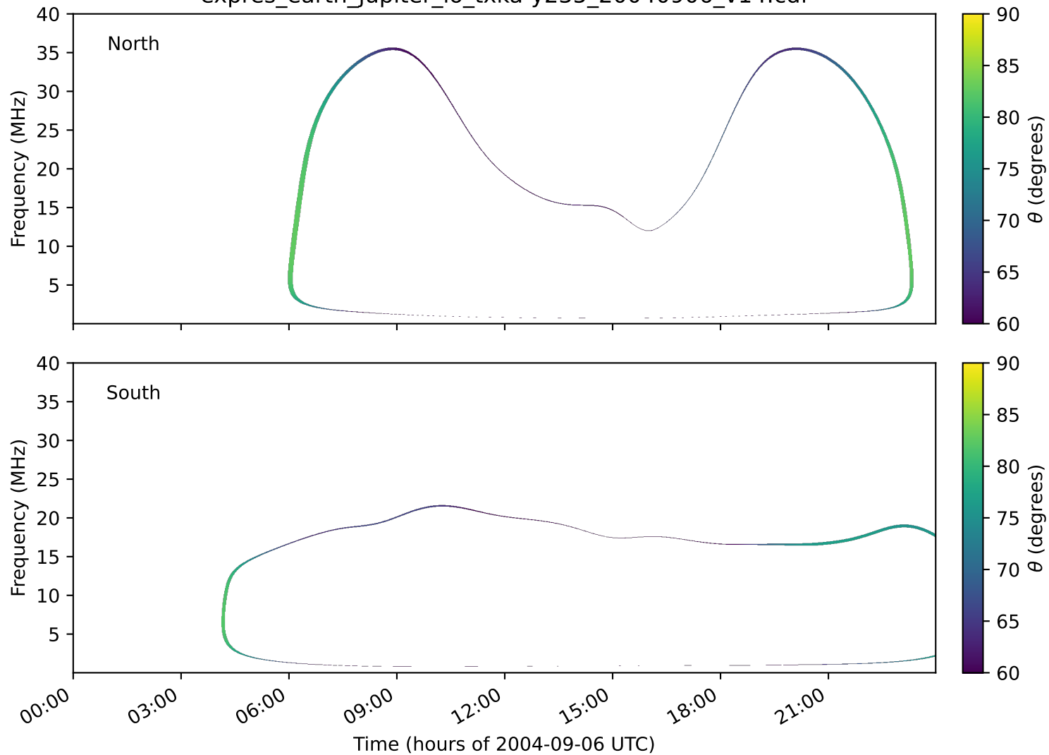
expres_earth_jupiter_io_txka-y235_20040906_v14.cdf
