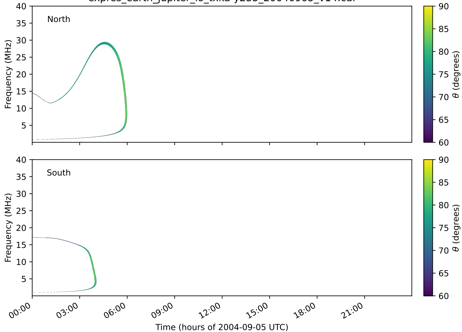
expres_earth_jupiter_io_txka-y235_20040905_v14.cdf
