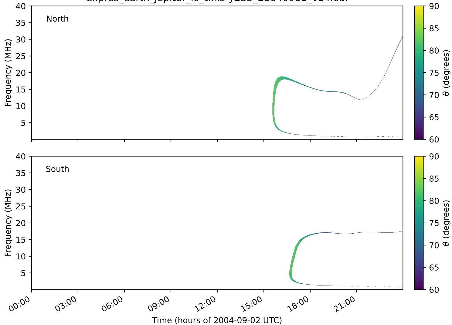
expres_earth_jupiter_io_txka-y235_20040902_v14.cdf
