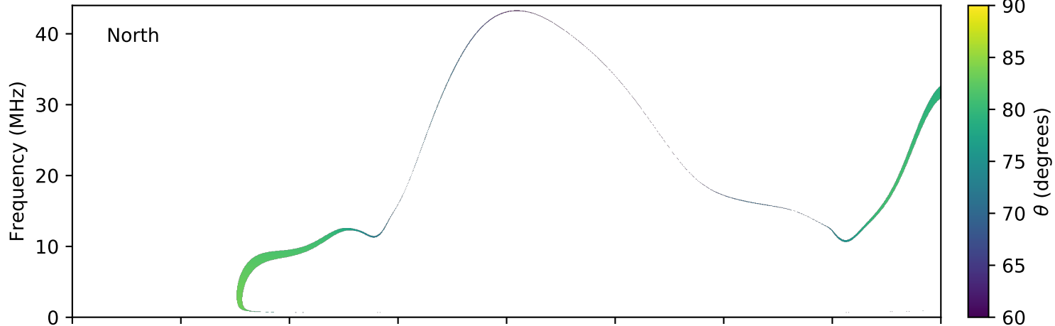
expres_earth_jupiter_io_jrm09_lossc-wid1deg_3kev_20040929_v11.cdf
