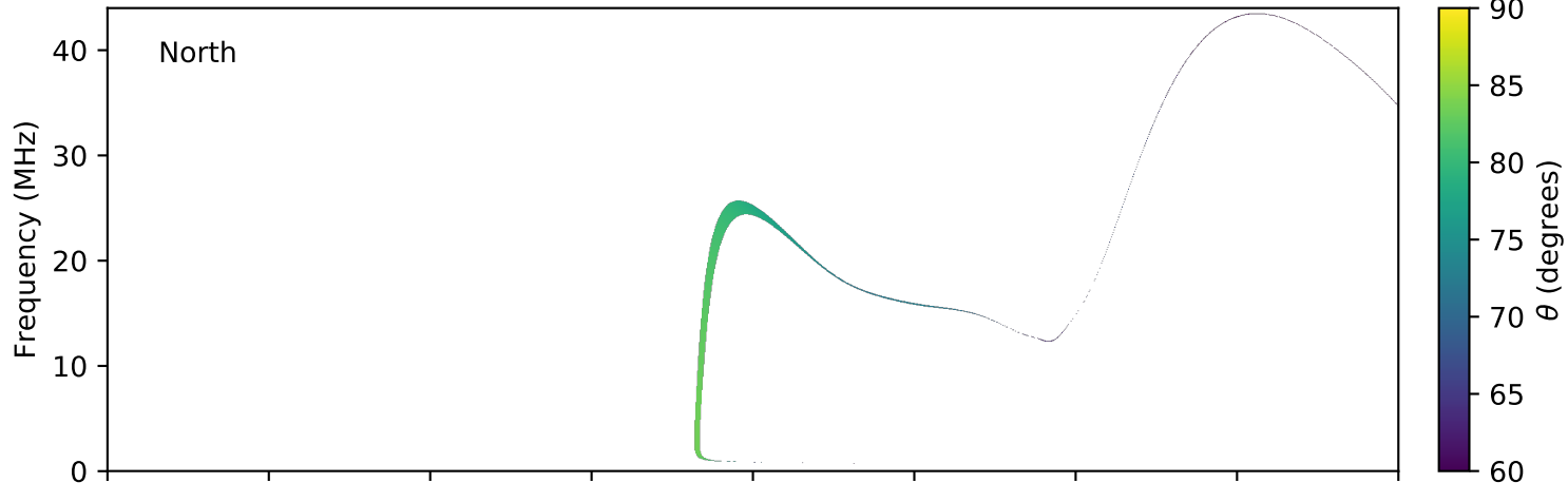
expres_earth_jupiter_io_jrm09_lossc-wid1deg_3kev_20040927_v11.cdf
