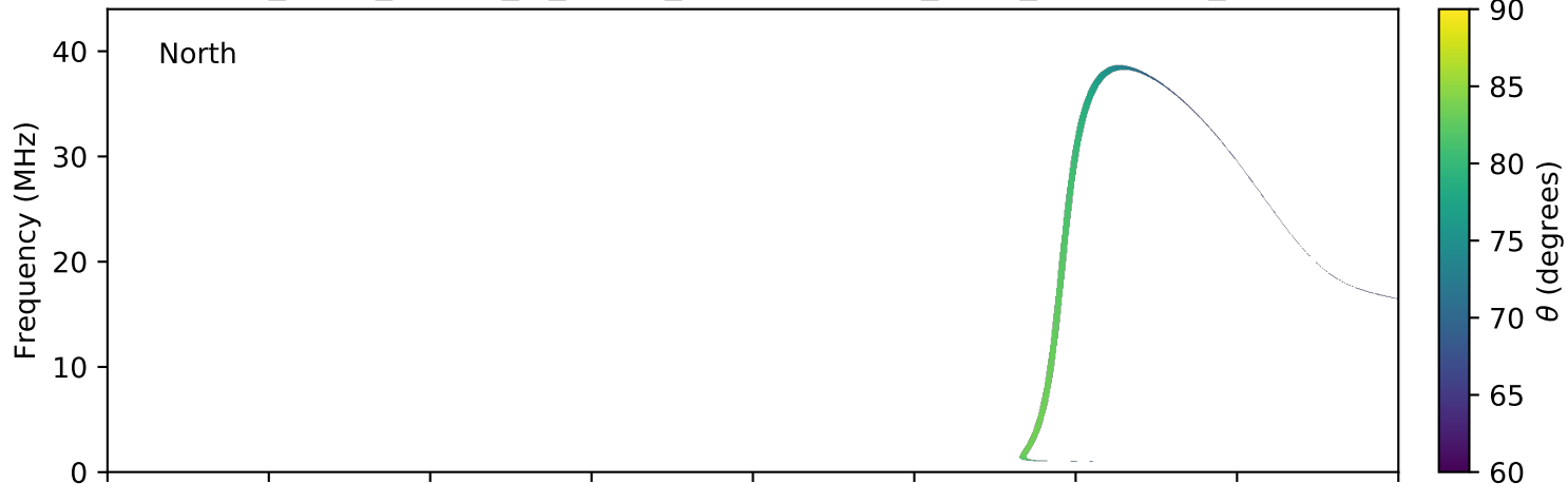
expres_earth_jupiter_io_jrm09_lossc-wid1deg_3kev_20040925_v11.cdf
