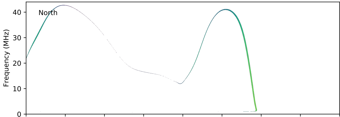
expres_earth_jupiter_io_jrm09_lossc-wid1deg_3kev_20040924_v11.cdf
