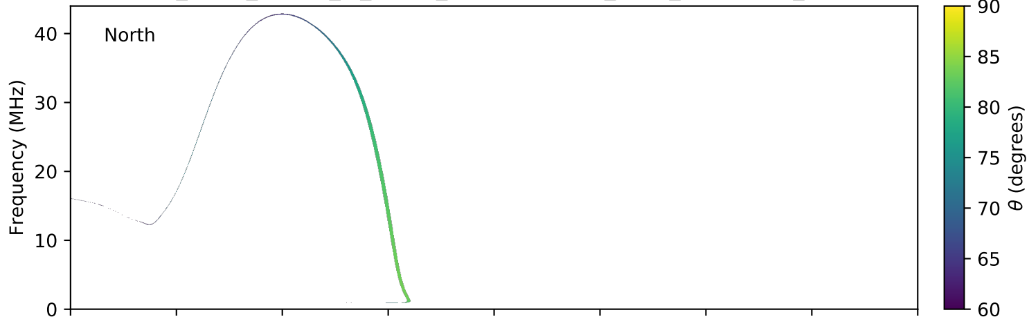
expres_earth_jupiter_io_jrm09_lossc-wid1deg_3kev_20040919_v11.cdf
