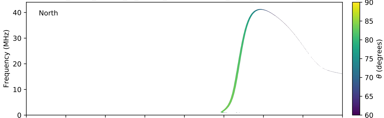
expres_earth_jupiter_io_jrm09_lossc-wid1deg_3kev_20040918_v11.cdf
