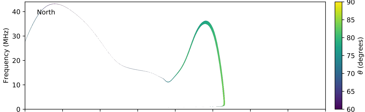
expres_earth_jupiter_io_jrm09_lossc-wid1deg_3kev_20040917_v11.cdf
