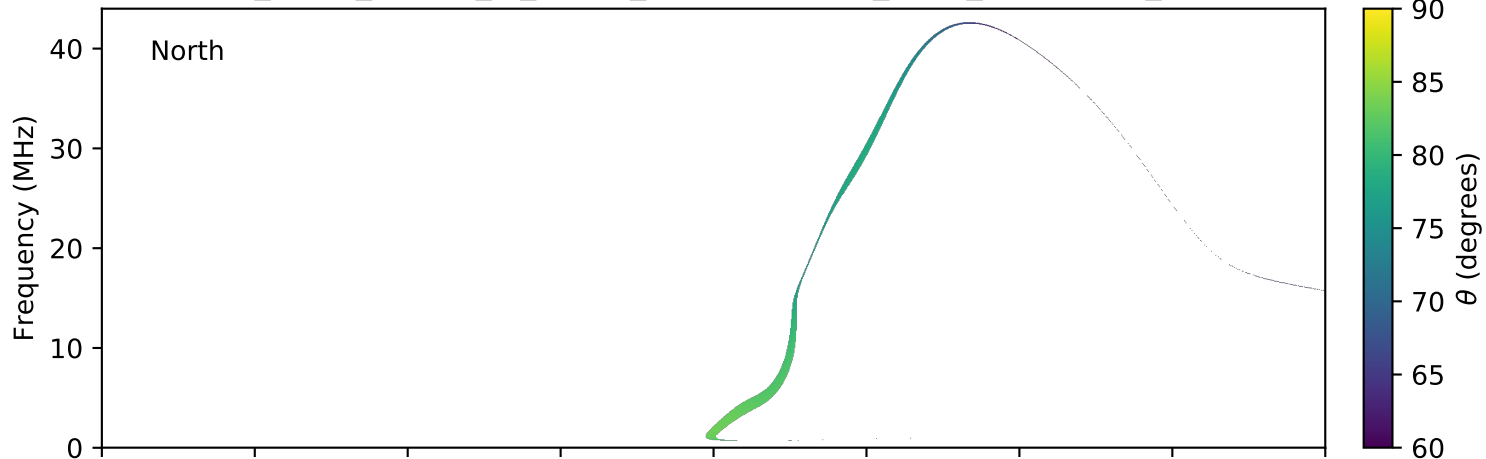
expres_earth_jupiter_io_jrm09_lossc-wid1deg_3kev_20040911_v11.cdf
