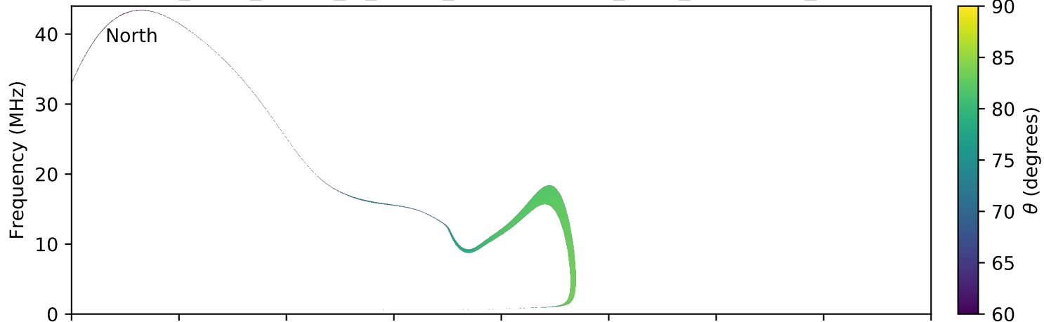
expres_earth_jupiter_io_jrm09_lossc-wid1deg_3kev_20040910_v11.cdf
