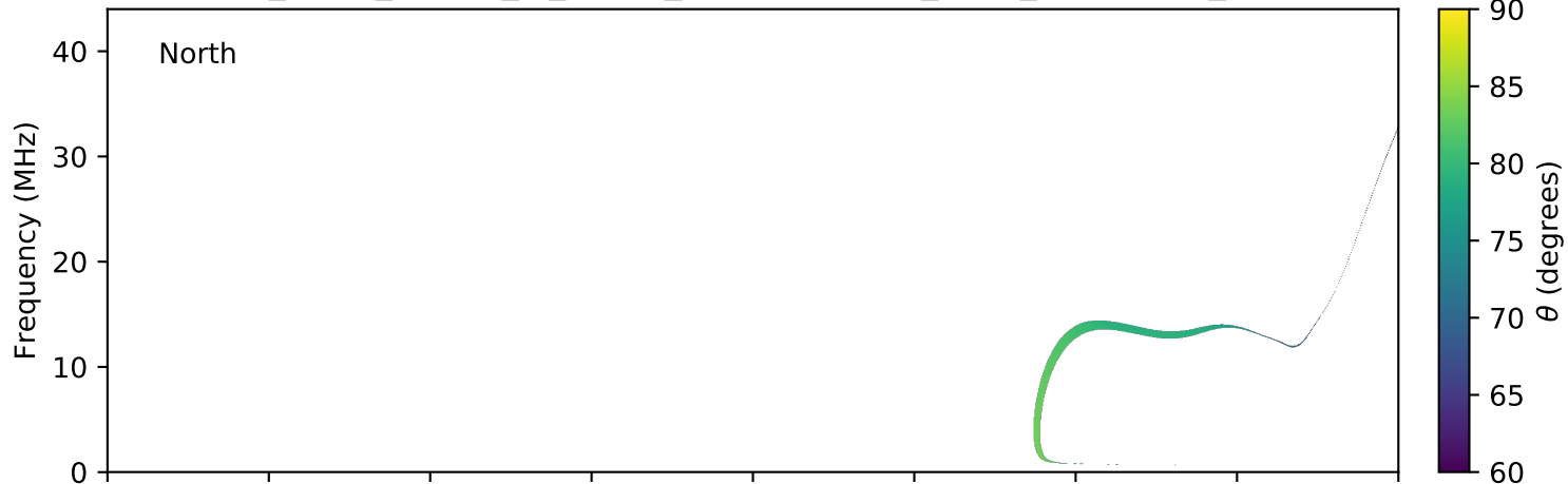
expres_earth_jupiter_io_jrm09_lossc-wid1deg_3kev_20040909_v11.cdf
