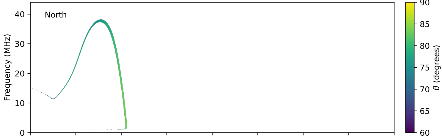
expres_earth_jupiter_io_jrm09_lossc-wid1deg_3kev_20040905_v11.cdf
