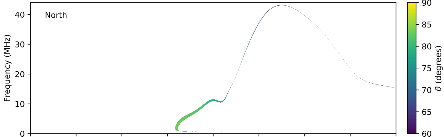
expres_earth_jupiter_io_jrm09_lossc-wid1deg_3kev_20040904_v11.cdf
