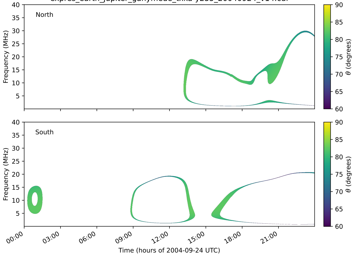
expres_earth_jupiter_ganymede_txka-y235_20040924_v14.cdf
