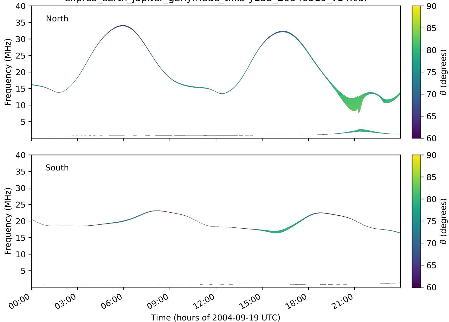
expres_earth_jupiter_ganymede_txka-y235_20040919_v14.cdf
