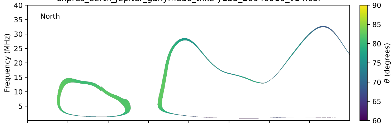
expres_earth_jupiter_ganymede_txka-y235_20040910_v14.cdf
