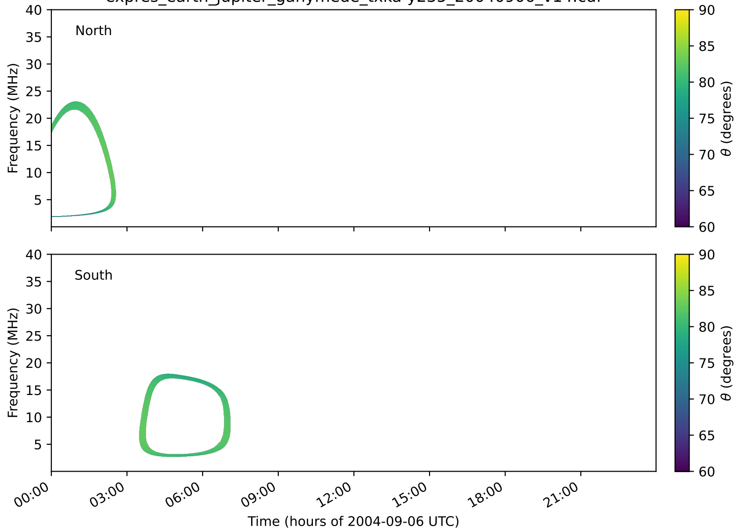
expres_earth_jupiter_ganymede_txka-y235_20040906_v14.cdf
