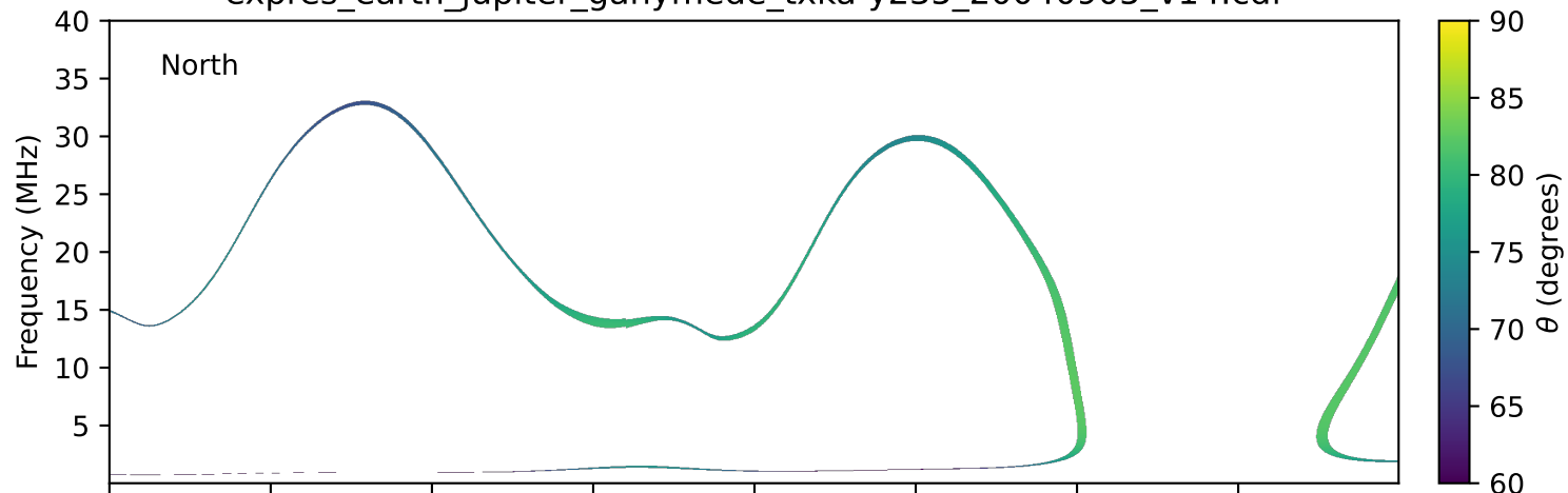
expres_earth_jupiter_ganymede_txka-y235_20040905_v14.cdf
