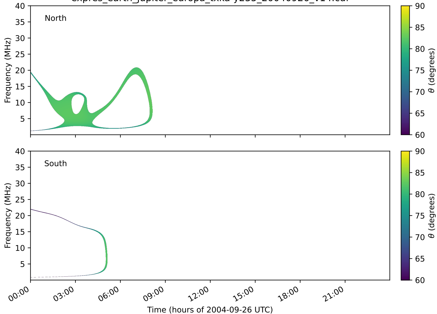
expres_earth_jupiter_europa_txka-y235_20040926_v14.cdf
