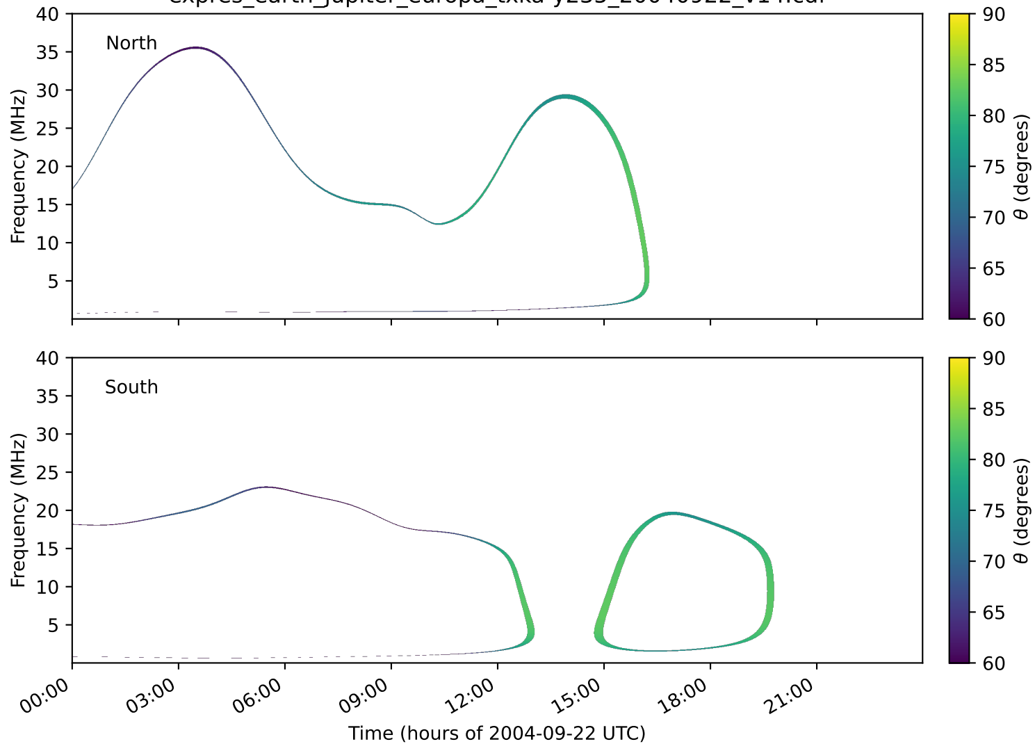
expres_earth_jupiter_europa_txka-y235_20040922_v14.cdf
