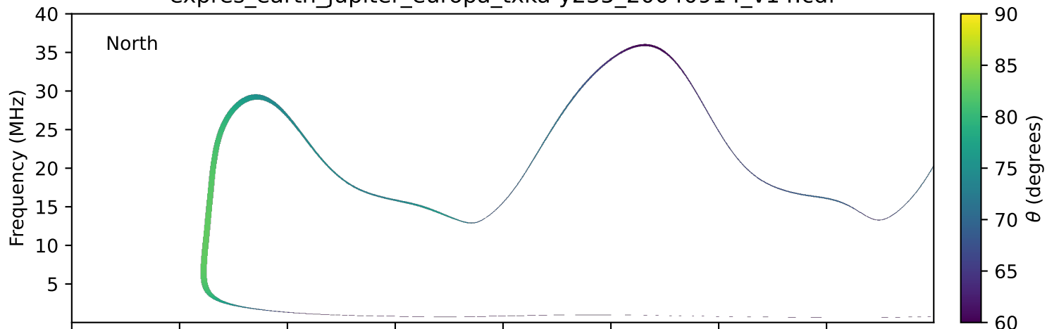
expres_earth_jupiter_europa_txka-y235_20040914_v14.cdf
