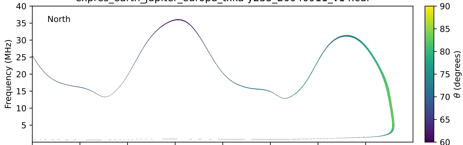
expres_earth_jupiter_europa_txka-y235_20040911_v14.cdf
