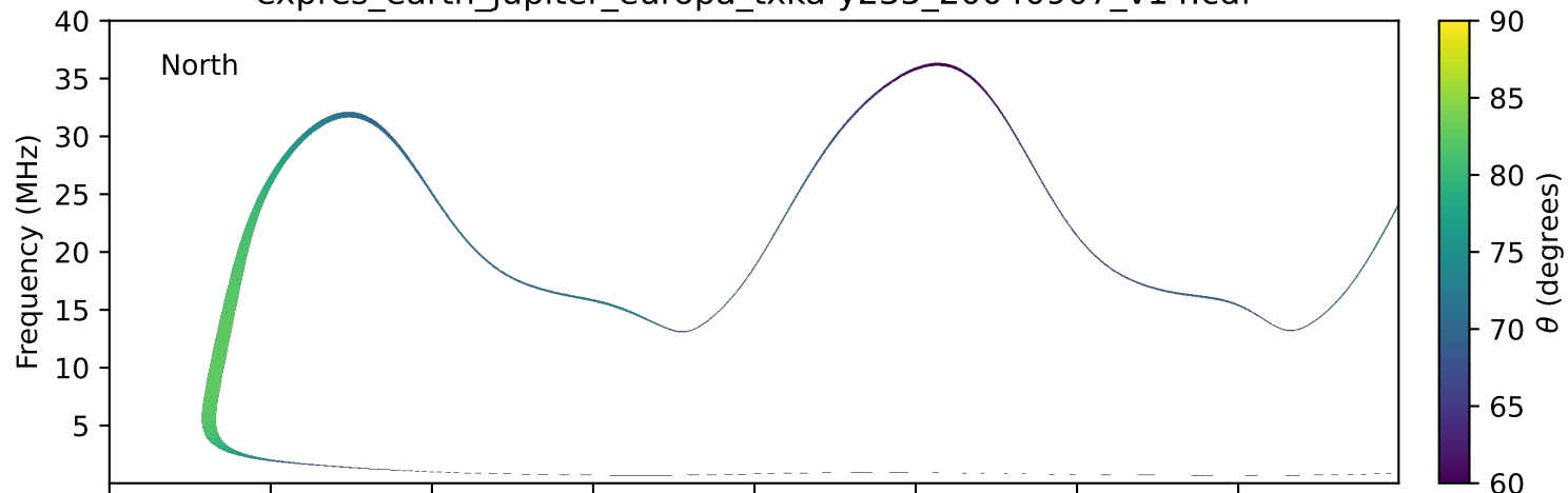
expres_earth_jupiter_europa_txka-y235_20040907_v14.cdf
