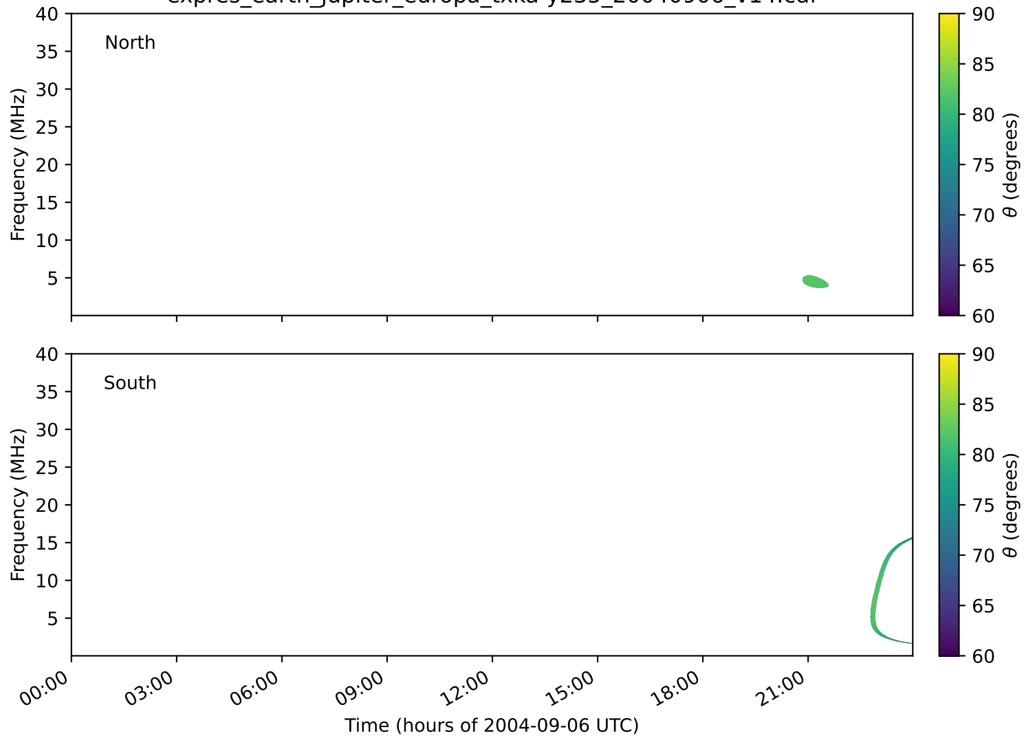
expres_earth_jupiter_europa_txka-y235_20040906_v14.cdf
