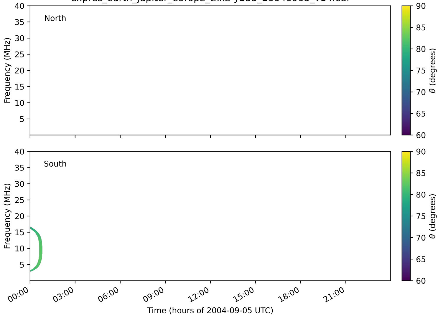
expres_earth_jupiter_europa_txka-y235_20040905_v14.cdf
