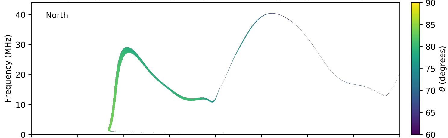
expres_earth_jupiter_europa_jrm09_lossc-wid1deg_3kev_20040921_v11.cdf
